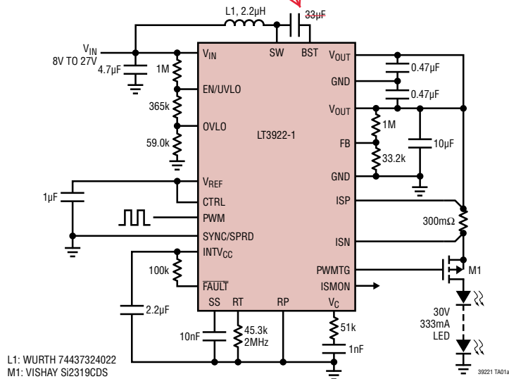
30V, 333mA Boost LED Driver with 25,000:1 PWM Dimming
